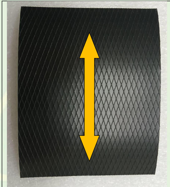
Test specimen orientation for testing (Vertical Direction)
